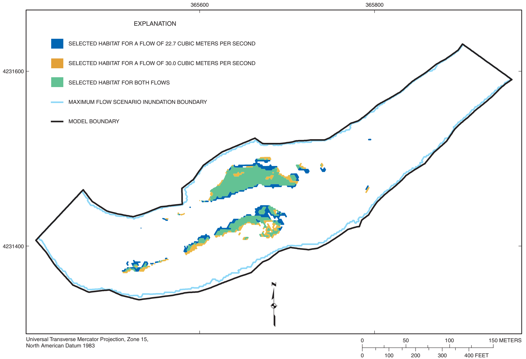
Figure 4-7. Selected habitat area distribution for habitat category 1 (suckermouth minnow) at flows of 22.7 and 30.0 cubic meters per second at Marais des Cygnes River site MDC2.
